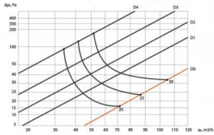
Canova Ø 100 (mandata / supply air)
