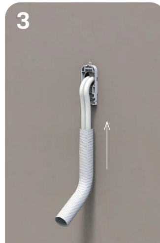
3 Place the refrigeration pipes and the power supply in the corrugated protection pipe
